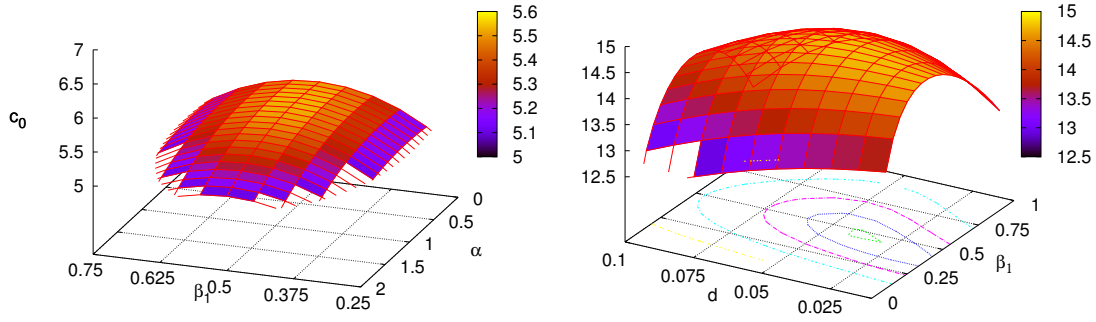
FIG. 2. Artificial network with degree-power/doubleton model (left) and the PFP and triangle model (right) showing c_0 .
